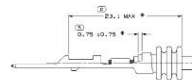
THREE RIB SEAL POSITION REF SCALE 5:1
