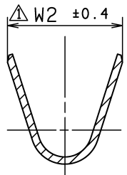
SEC. M-M
