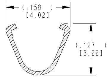
SECTION A-A WIRE BARREL
