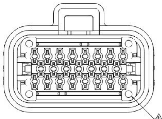
BOTTOM VIEW WITH LOCKING WEDGE
