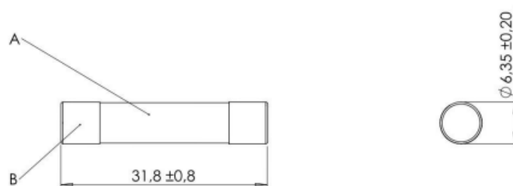
A Glass tube B Nickel plated caps with voltage and nominal rating marking
