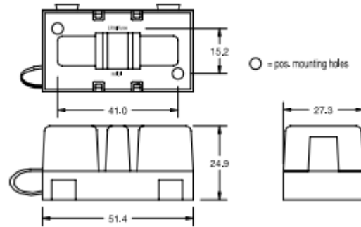
Dimensions in mm / Maße in mm
